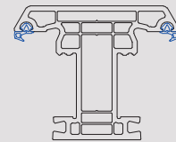
102268 86mm T Mullion
