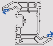
103364 82mm Tilt N Turn Sash
