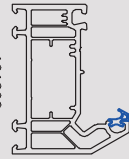
101308 59mm Outerframe
