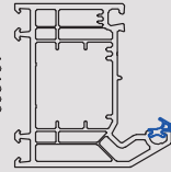
101309 67mm Outerframe
