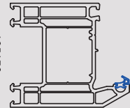
105176 80mm Outerframe
