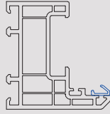
701591 68mm Outerframe
